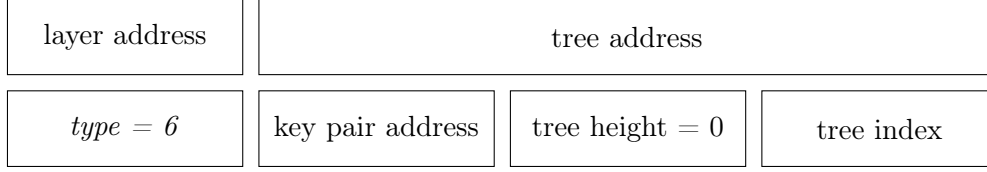
Figure 8: FORS key generation address.
