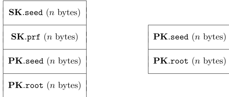
Figure 14: Left: SPHINCS + secret key. Right: SPHINCS + public key.
