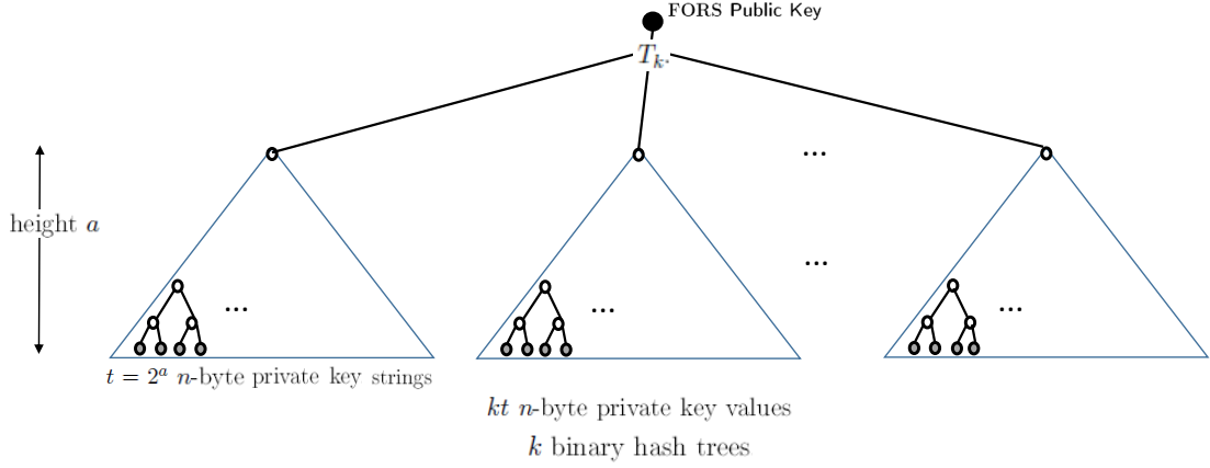
Figure 12: FORS trees and PK
