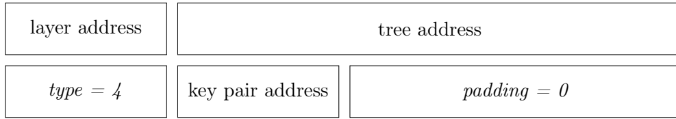
Figure 6: FORS tree roots compression address.
