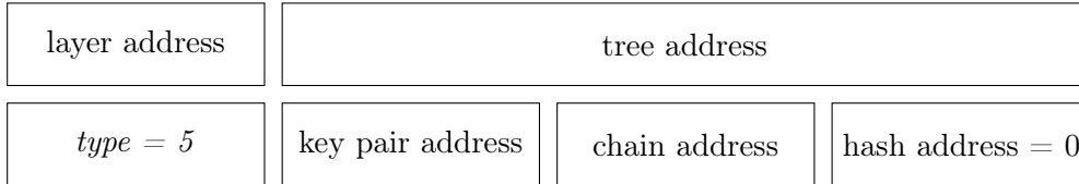
Figure 7: WOTS + key generation address.
